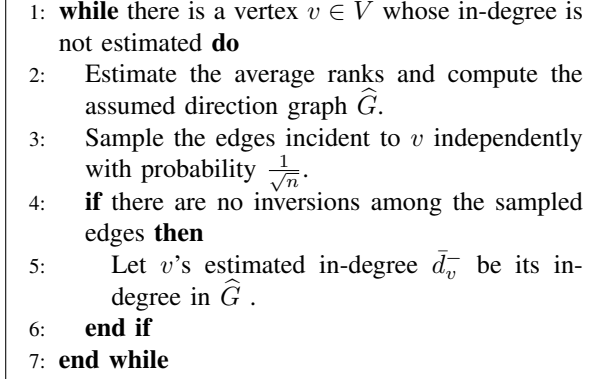
Figure 2. Algorithm INIT-SAMPLE
